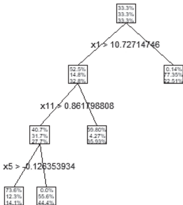
Fig. 2. Decision tree
