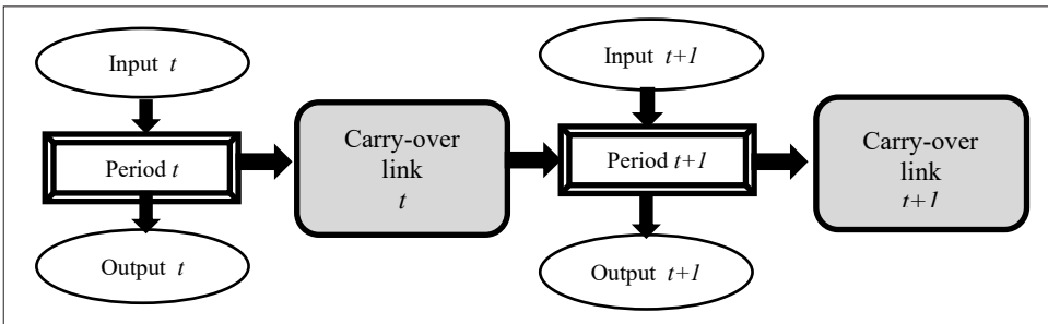
Figure 1. Structure of the dynamic SBM model
