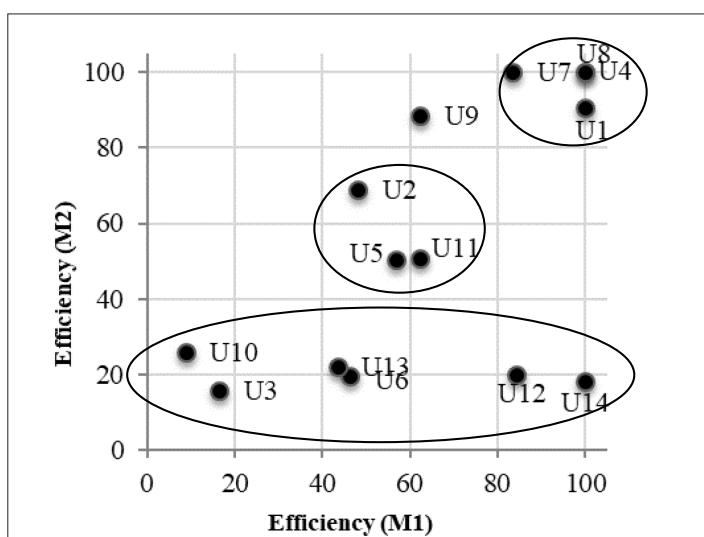
Figure 4. Benchmarking of total efficiency in M1 and M2
