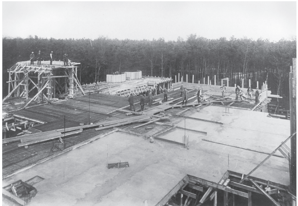
Fig. 5. “Zonnestraal” sanatorium, main building during construction around 1927. The concrete slurry was mixed by hand which resulted in inhomogeneity, which was worsened by the onsite transportation in small batches by wheel barrows (right) (photographer unknown, from Duiker’s personal archive, coll. Jelles and Alberts, HNI Rotterdam)
