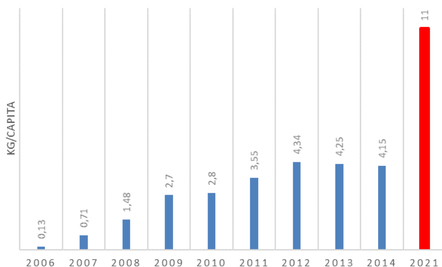
Figure 2. WEEE collected per capita in Poland
