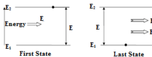
Figure 5. Stimulated Radiation
