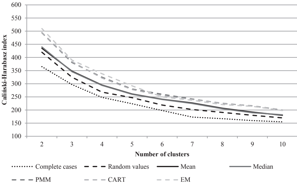
Fig. 3. Calinski-Harabasz index values for different imputation methods – k-means method
