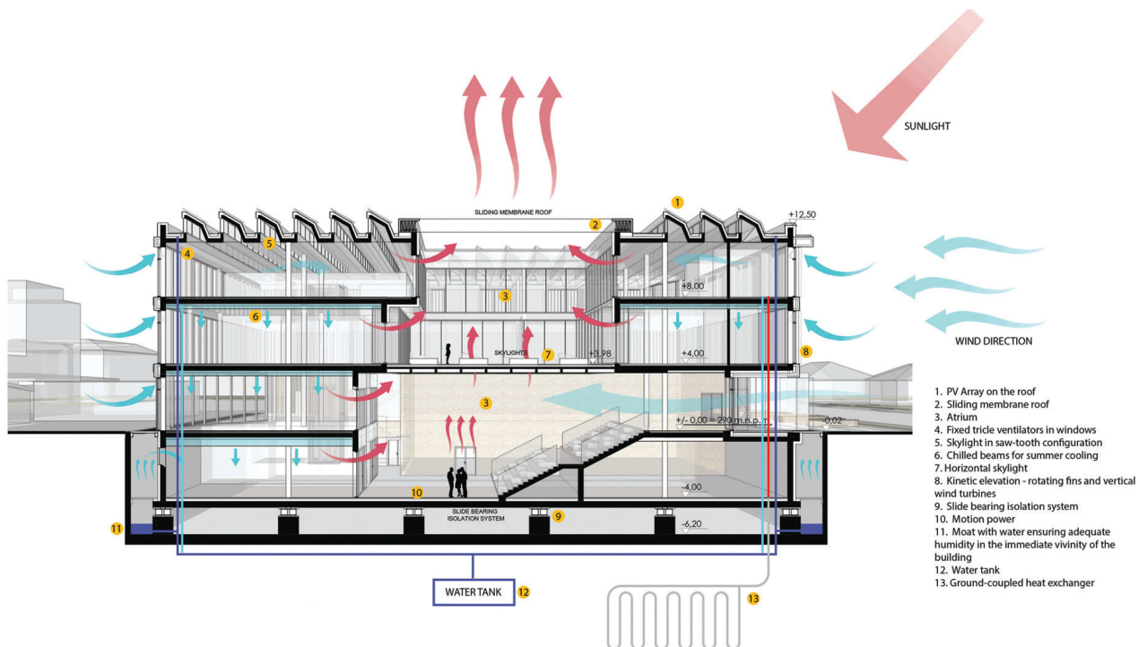
Fig. 8. Graphic section and air circulation process (elaborated by A. Kaczmarek)
