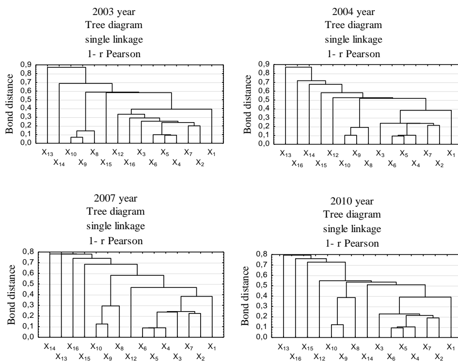
Fig. 1. Clustering results by the method of single linkage, respectively for 2003, 2004, 2007 and 2010
