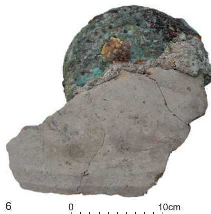
10. Masafi-1, Phase 1a, the pit with basin MSF-2133 half-buried inside, possibly a first combustion structure: 1, 2, 5. the pit in course of excavation with the basin in situ ; 3, 6. sample 156-44 comprising three ingots stuck on potsherds belong to basin MSF-2133, found inside jar MSF-2098, in Phase 1b; 4. drawing of the basin (Phot. A. Hamel, C. Le Carlier; drawing: V. Bernard).
