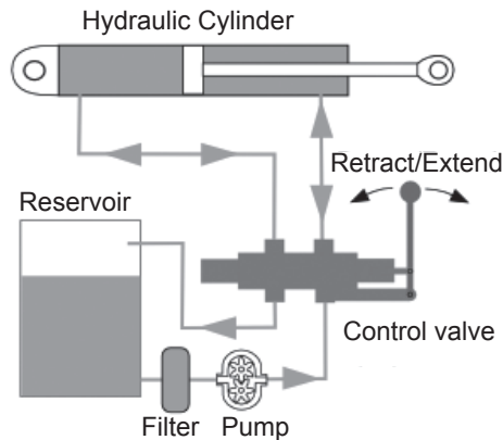
Fig. 1. basic hydrostatic drive system. Author: Duk, source: Wikimedia Commons, license: CC-BY-SA-3.0
