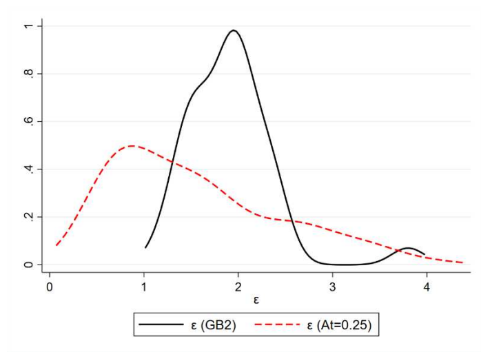
Figure 11. The density functions of \epsilon based on the GB2 for the years 1998–2000 and \epsilon based on NRSI (Atkinson index=0.25)
