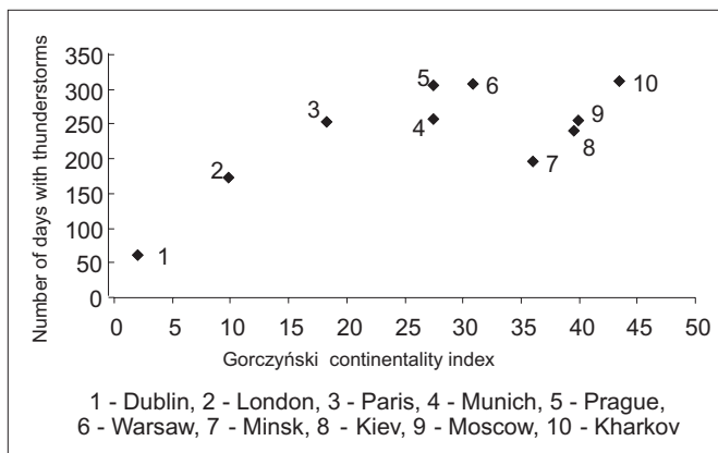
Fig. 2. Dependence of the long-term number of days with thunderstorms on the Gorceżyński continentality index in selected European cities (1994–2005).
