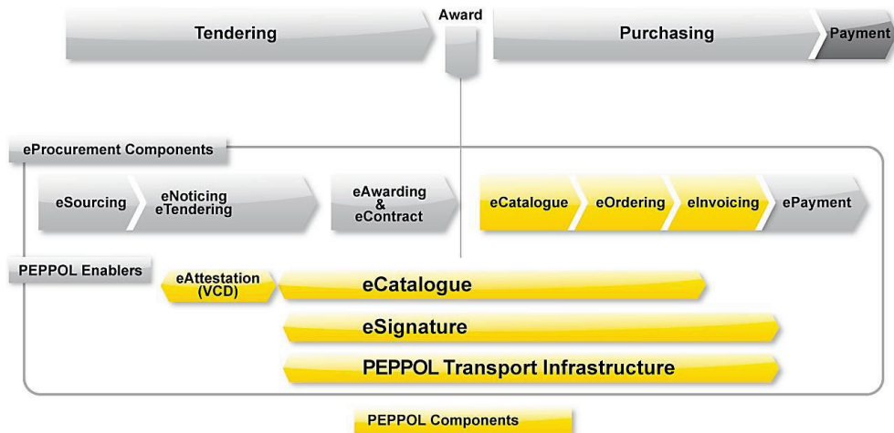
Figure 4. PEPPOL components
