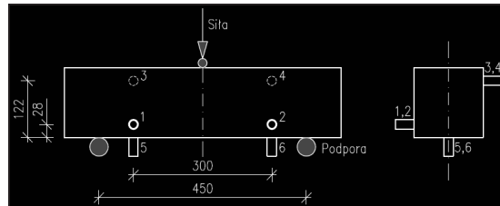
Fig. 3. The spacing of measuring-sensors to the Sigma analysis, numbers 1–6 are sensors (own elaboration)
