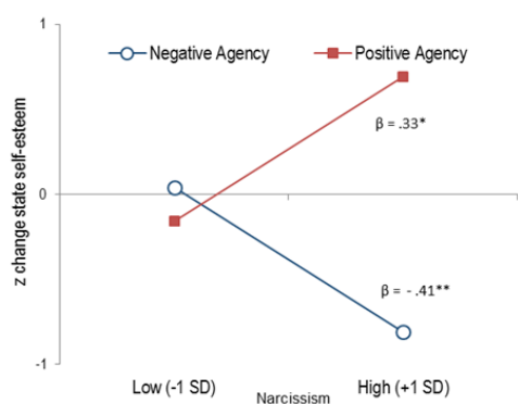
Figure 3. Z - State self-esteem (post– pre feedback state self-esteem) as a function of agency (negative vs. positive) feedback and narcissism. High and low levels of narcissism were designated using values at 1 SD below and 1 SD above the mean NPI.
