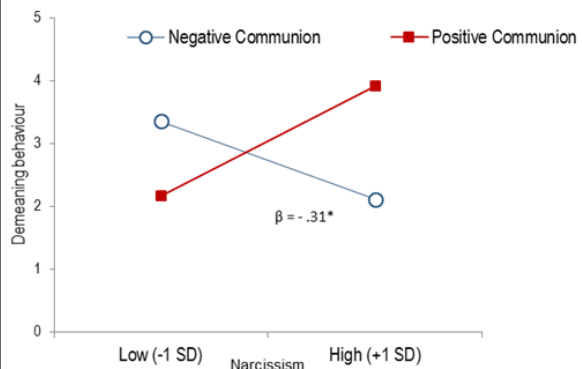
Figure 1. Demeaning behaviour as a function of communal (negative vs. positive) feedback and narcissism. High and low levels of narcissism were designated using values at 1 SD below and 1 SD above the mean NPI.
