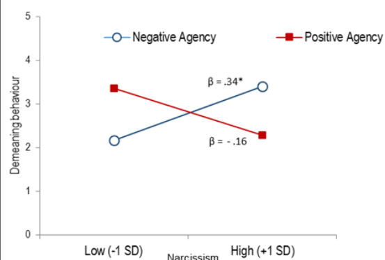
Figure 2. Demeaning behaviour as a function of agency (negative vs. positive) feedback and narcissism. High and low levels of narcissism were designated using values at 1 SD below and 1 SD above the mean NPI.
